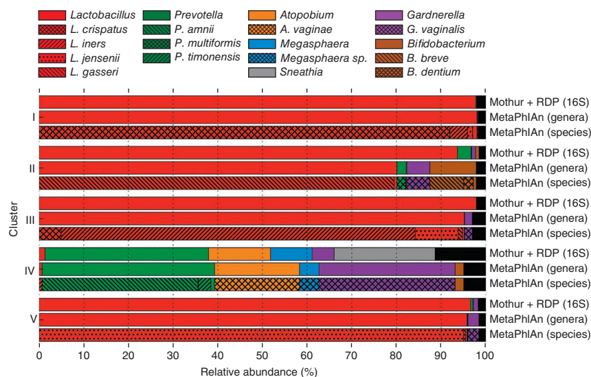
Figure 2 | Composition of healthy vaginal microbiota. MetaPhlAn species and genus abundances and 16S phylotype abundances for 51 healthy vaginal microbiomes from the Human Microbiome Project are shown. Samples were naively grouped by assigning each based on its dominant (>50%) Lactobacillus species or by the absence (<2%) of any Lactobacillus . For each cluster (named from I to V 5 ) we report averages across samples for all genera and species as inferred by MetaPhlAn and, for genera, as estimated by the combination of the mothur 16S rRNA processing pipeline and the Ribosomal Database Project (RDP) classifier (see Online Methods) applied to 16S rRNA gene sequences from the same specimen.
